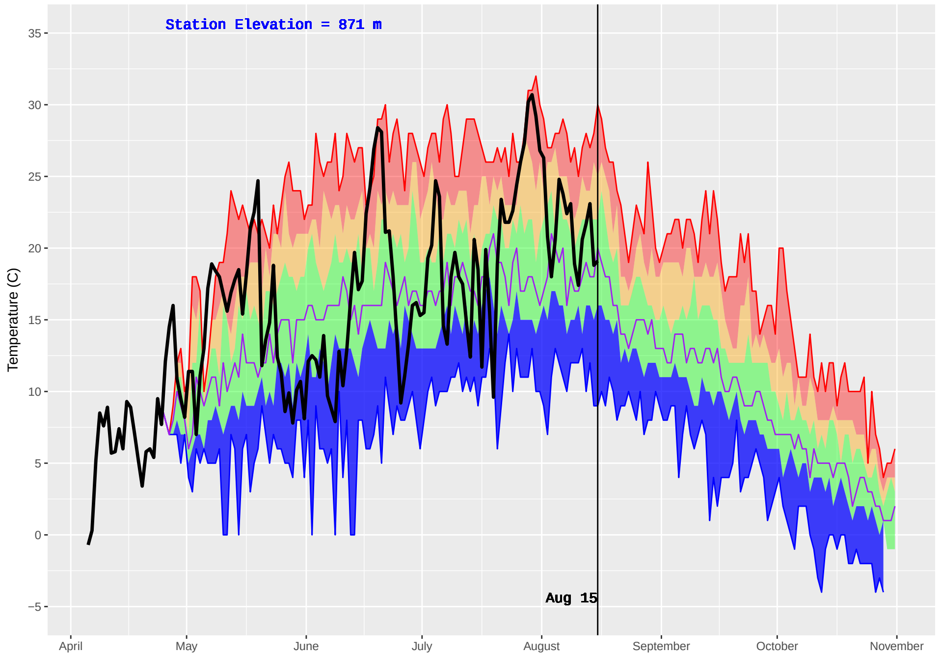
SUSTUT (156) : Historical (1989–2016) and Current (2018) Daily Temperature
