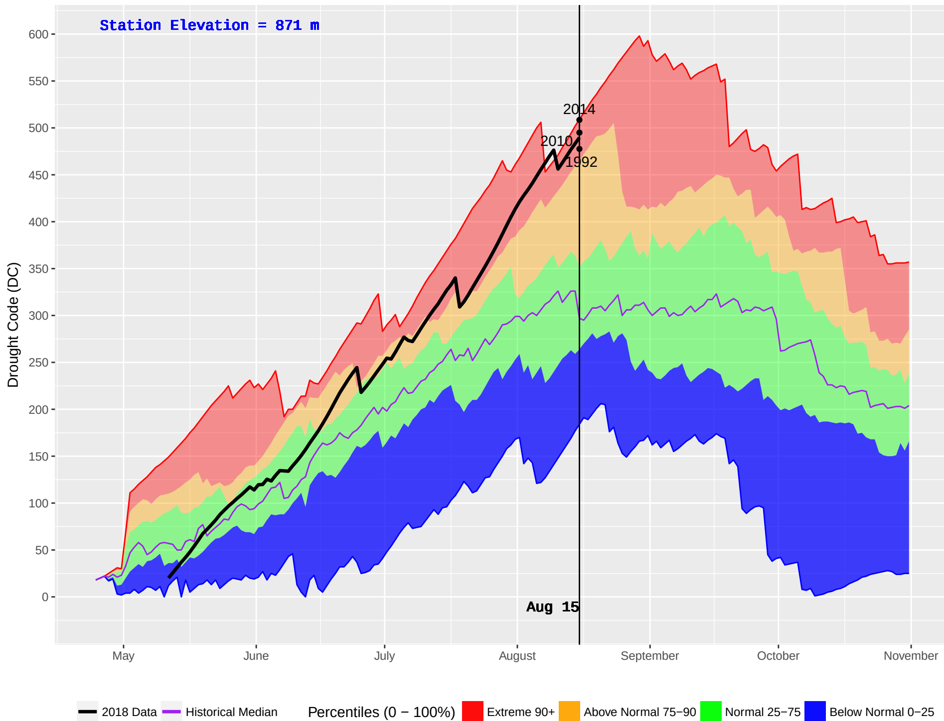
SUSTUT (156) : Historical (1989–2016) and Current (2018) Daily Drought Code (DC)
