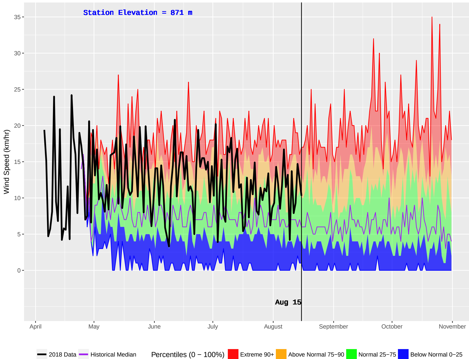
SUSTUT (156) : Historical (1989–2016) and Current (2018) Daily Wind Speed
