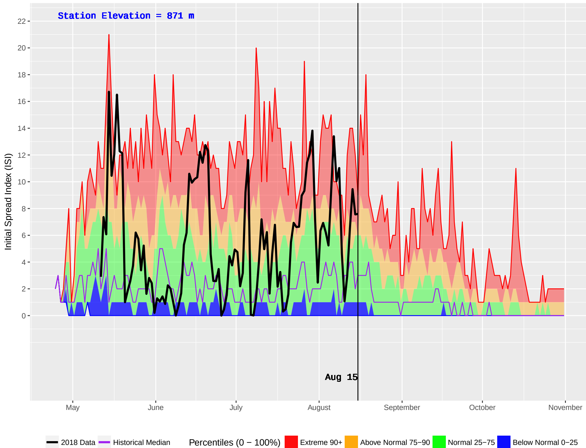
SUSTUT (156) : Historical (1989–2016) and Current (2018) Daily Initial Spread Index (ISI)
