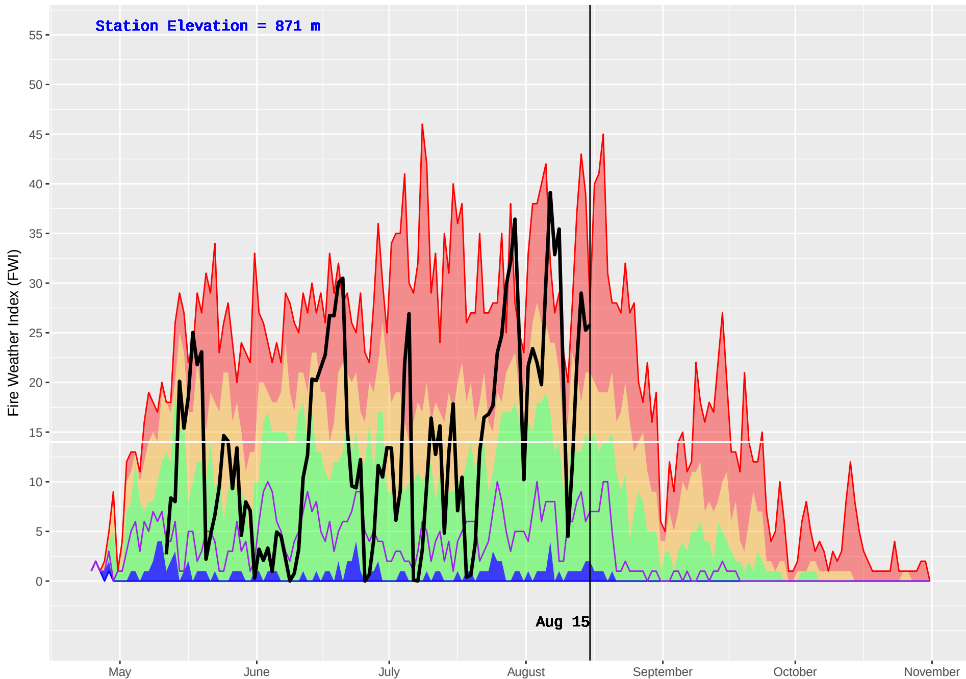
SUSTUT (156) : Historical (1989–2016) and Current (2018) Daily Fire Weather Index (FWI)
