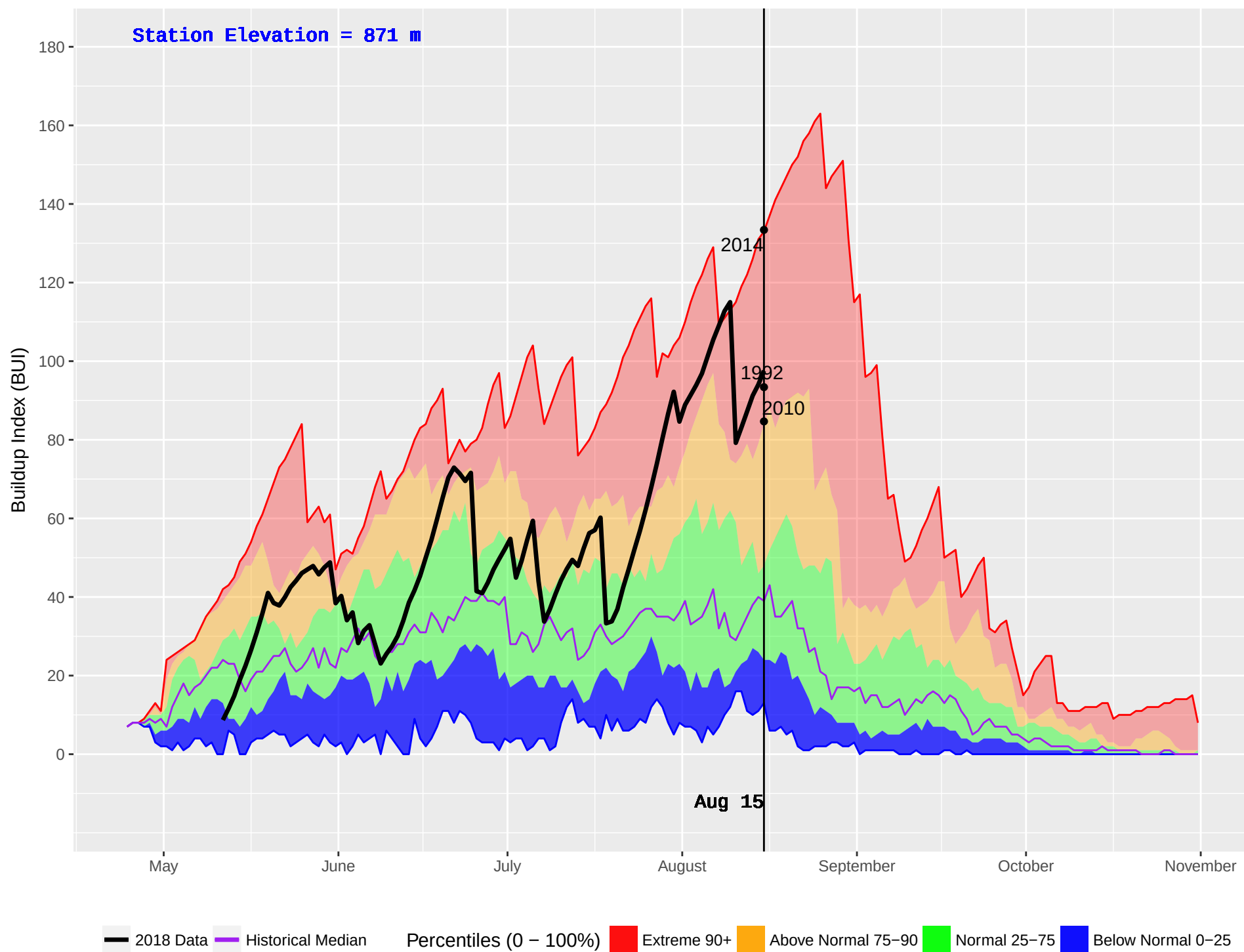
SUSTUT (156) : Historical (1989–2016) and Current (2018) Daily Buildup Index (BUI)
